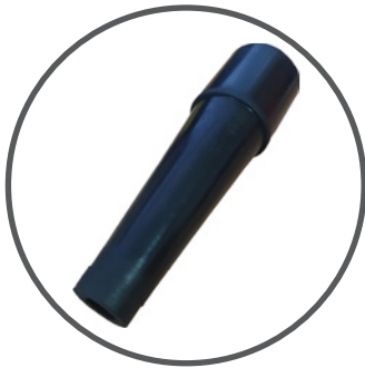
Replacement Nozzle 1.5"/38mm Internal Diameter P/N: 180014
